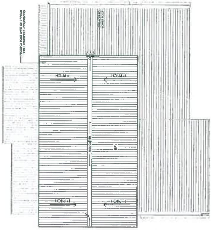
1 ROOF PLAN - UPPER A-200 1:100
